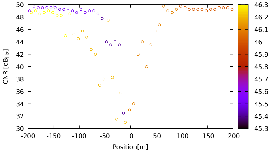
CNR vs position for G01 (L2) on LeicaGS18 - DOY 263 jam. 3
