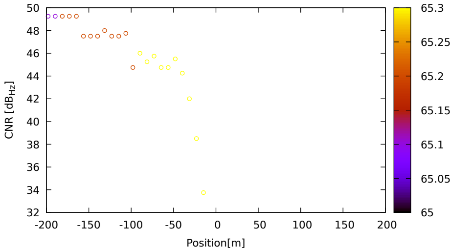
CNR vs position for G04 (L1) on LeicaGS18 - DOY 263 jam. 2
