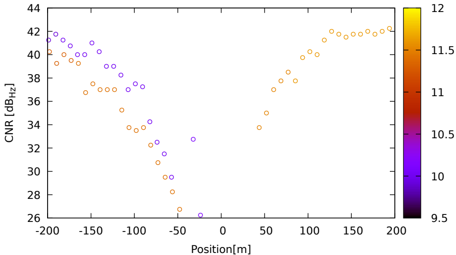
CNR vs position for G06 (L1) on LeicaGS18 - DOY 263 jam. 1
