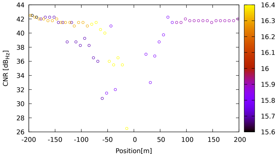
CNR vs position for G06 (L1) on LeicaGS18 - DOY 263 jam. 3
