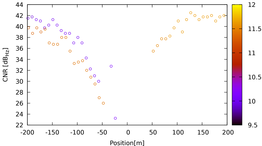
CNR vs position for G06 (L2) on LeicaGS18 - DOY 263 jam. 1
