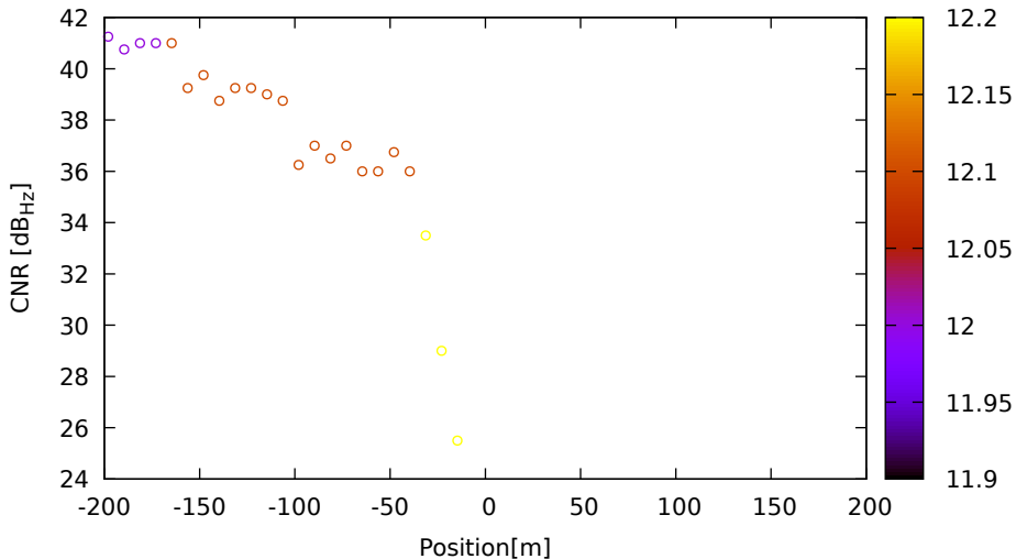
CNR vs position for G06 (L2) on LeicaGS18 - DOY 263 jam. 2
