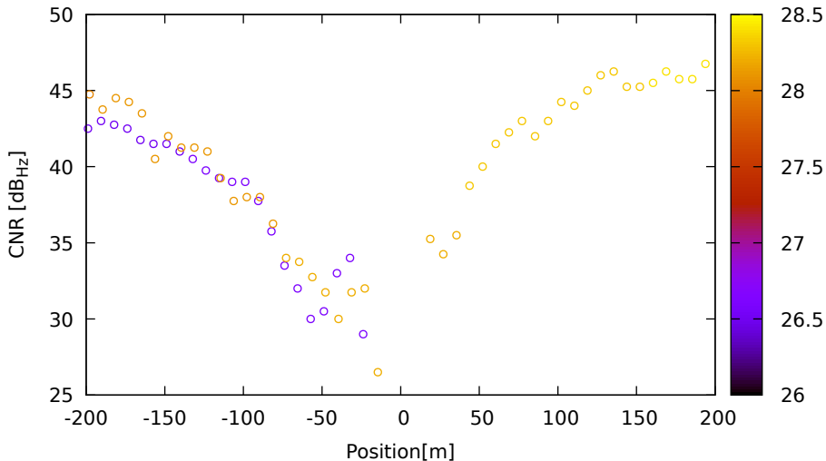
CNR vs position for G09 (L2) on LeicaGS18 - DOY 263 jam. 1
