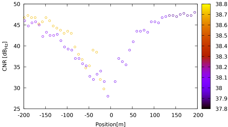
CNR vs position for G17 (L2) on LeicaGS18 - DOY 263 jam. 1
