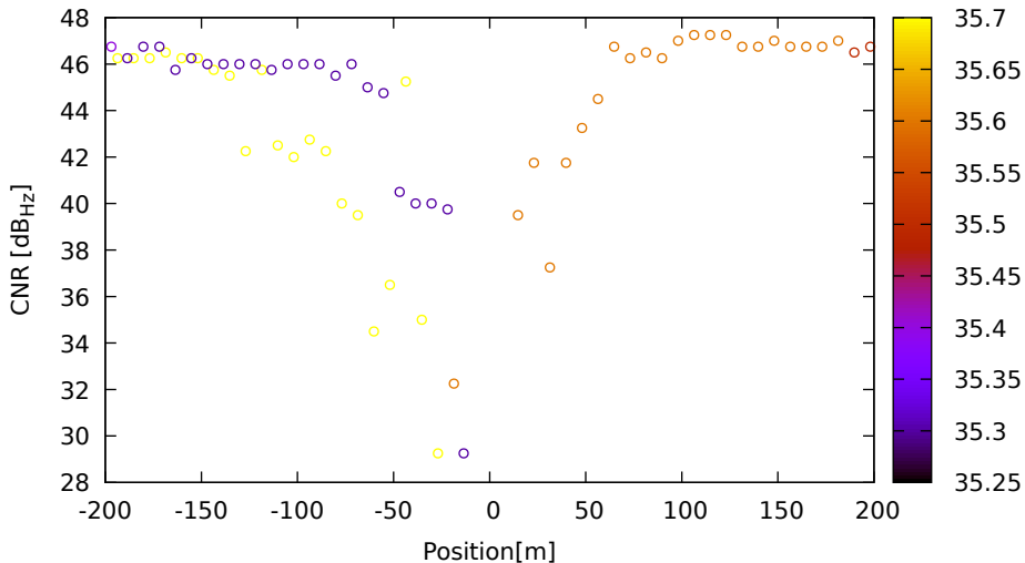
CNR vs position for G17 (L2) on LeicaGS18 - DOY 263 jam. 3
