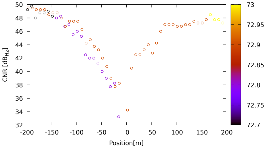
CNR vs position for R02 (G2) on LeicaGS18 - DOY 263 jam. 1
