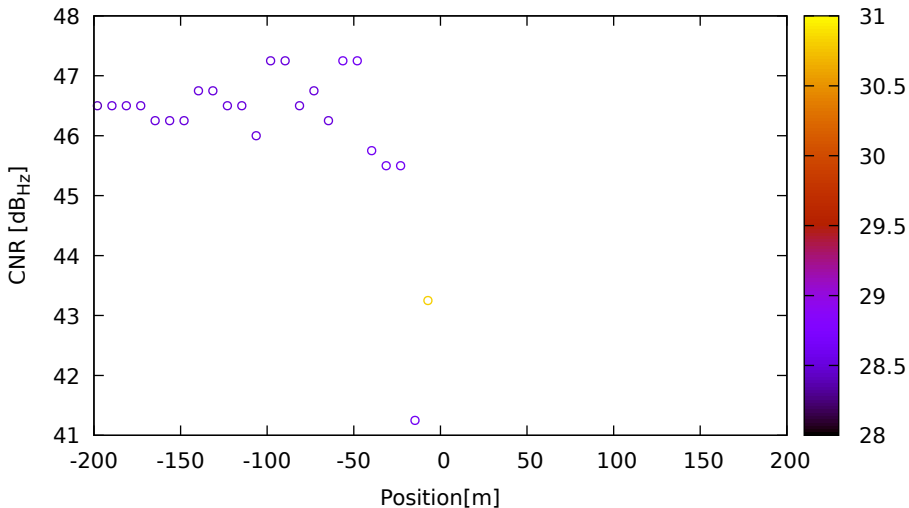
CNR vs position for R03 (G1) on LeicaGS18 - DOY 263 jam. 2
