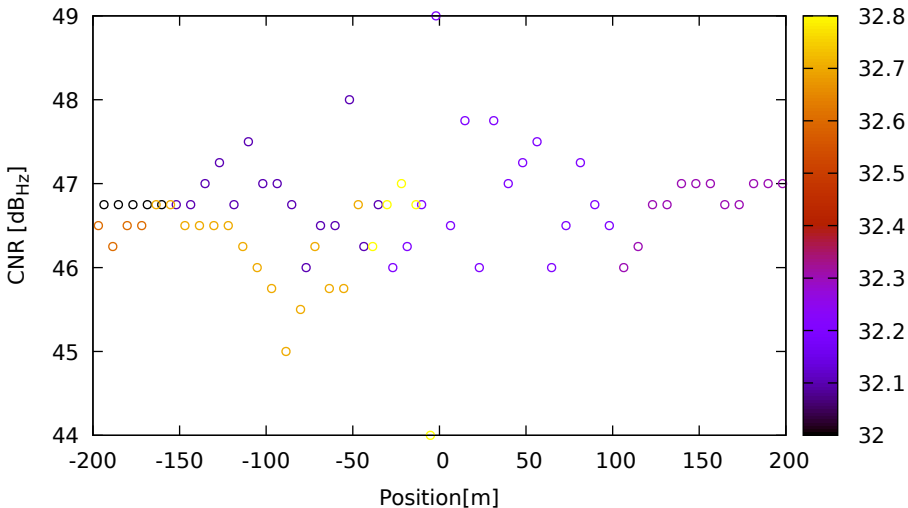
CNR vs position for R03 (G1) on LeicaGS18 - DOY 263 jam. 3
