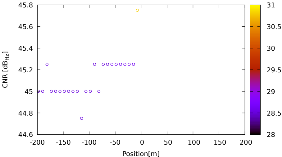
CNR vs position for R03 (G2) on LeicaGS18 - DOY 263 jam. 2
