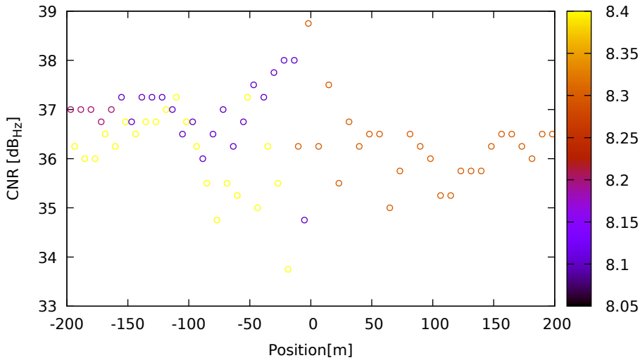
CNR vs position for R10 (G1) on LeicaGS18 - DOY 263 jam. 3
