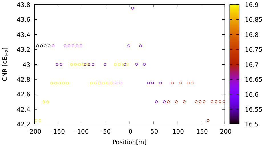
CNR vs position for R11 (G2) on LeicaGS18 - DOY 263 jam. 3
