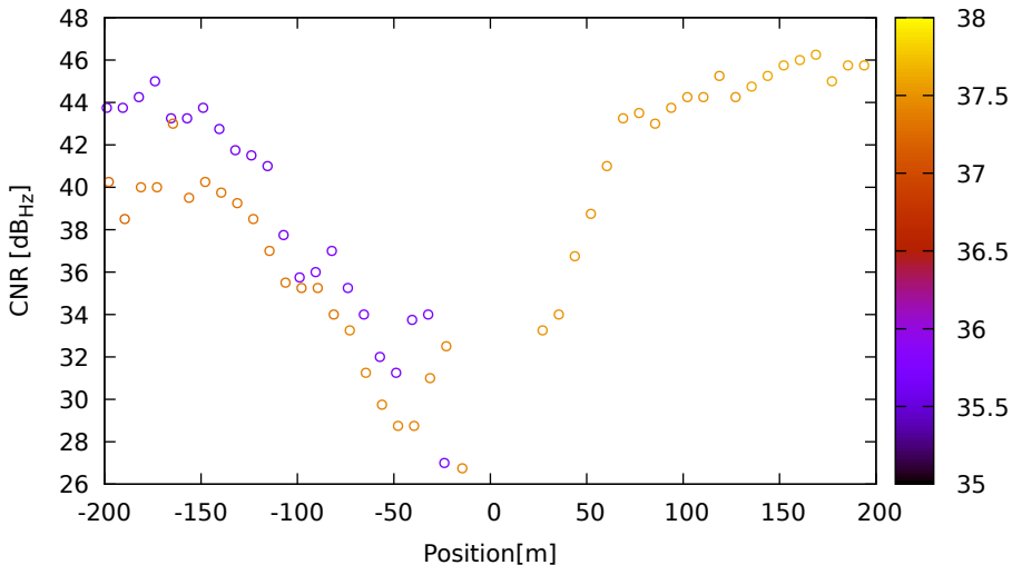
CNR vs position for R18 (G1) on LeicaGS18 - DOY 263 jam. 1
