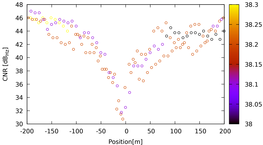
CNR vs position for C09 (B2) on LeicaGS18 - DOY 263 jam. 1
