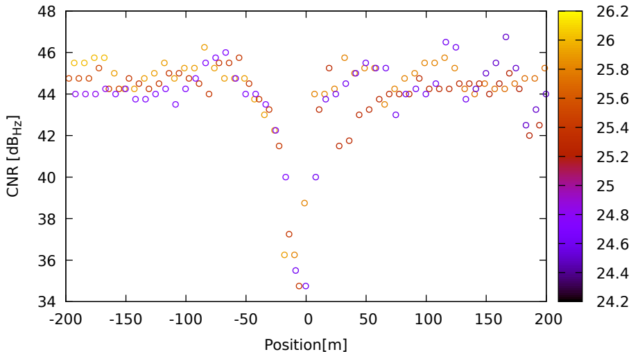
CNR vs position for C21 (B3) on LeicaGS18 - DOY 263 jam. 1
