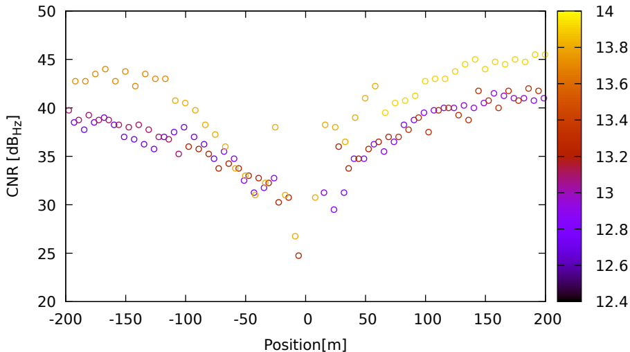
CNR vs position for C26 (B1) on LeicaGS18 - DOY 263 jam. 1
