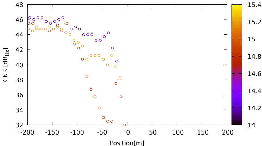
CNR vs position for C26 (B1) on LeicaGS18 - DOY 263 jam. 2
