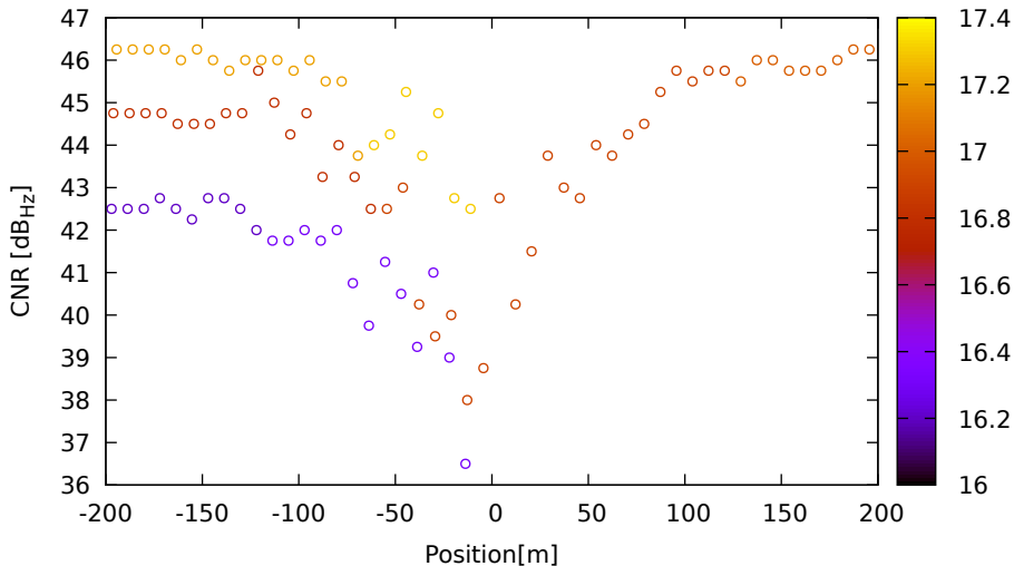
CNR vs position for C26 (B1) on LeicaGS18 - DOY 263 jam. 3
