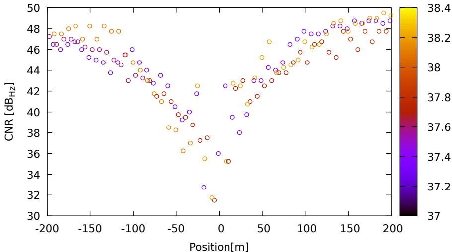
CNR vs position for C28 (B1) on LeicaGS18 - DOY 263 jam. 1
