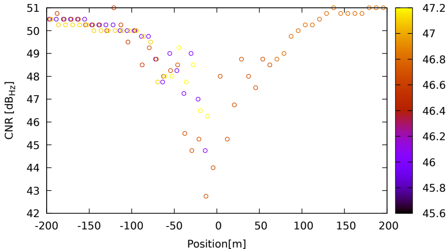
CNR vs position for C33 (B1) on LeicaGS18 - DOY 263 jam. 3
