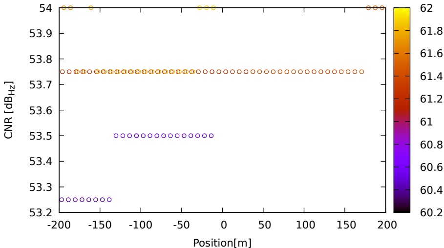
CNR vs position for E04 (E5b) on LeicaGS18 - DOY 263 jam. 3
