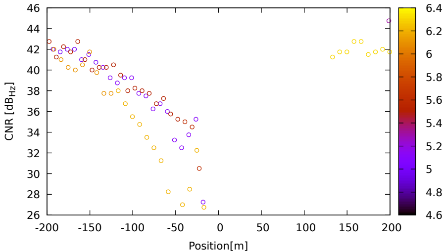
CNR vs position for E09 (E1) on LeicaGS18 - DOY 263 jam. 1
