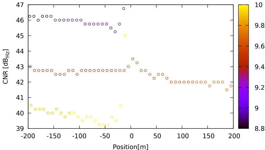
CNR vs position for E09 (E5a) on LeicaGS18 - DOY 263 jam. 3
