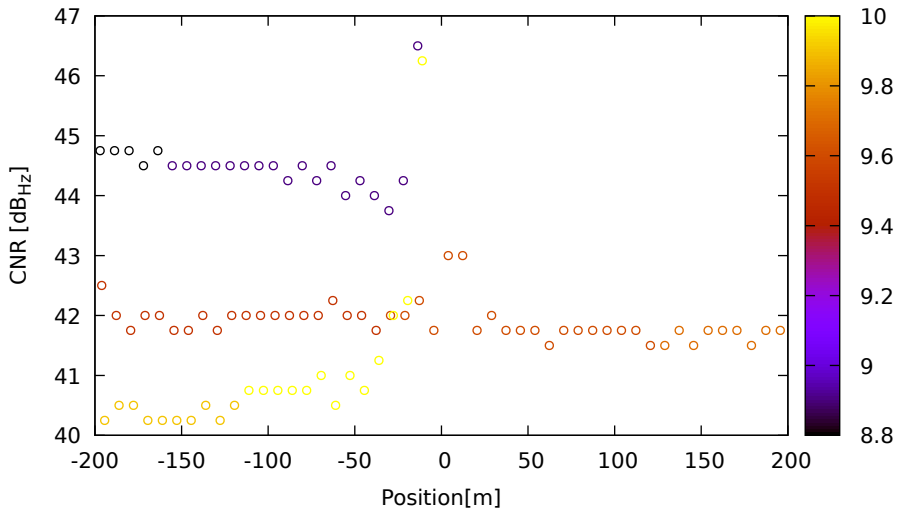
CNR vs position for E09 (E5b) on LeicaGS18 - DOY 263 jam. 3
