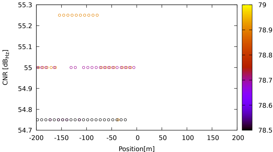
CNR vs position for E10 (E5b) on LeicaGS18 - DOY 263 jam. 2
