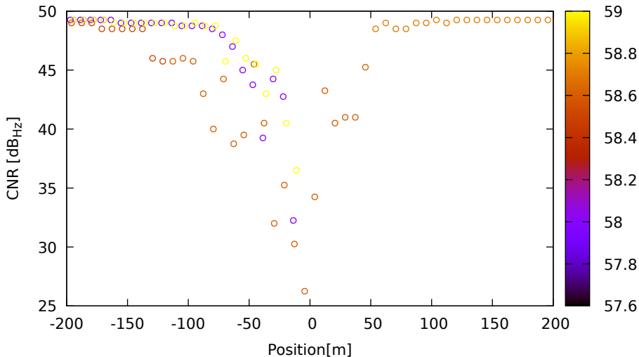
CNR vs position for E11 (E1) on LeicaGS18 - DOY 263 jam. 3
