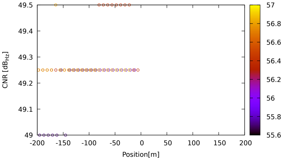
CNR vs position for E11 (E5a) on LeicaGS18 - DOY 263 jam. 2
