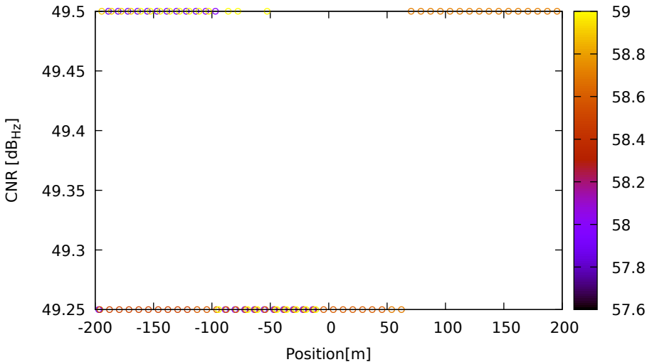
CNR vs position for E11 (E5a) on LeicaGS18 - DOY 263 jam. 3
