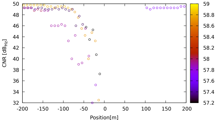
CNR vs position for E12 (E1) on LeicaGS18 - DOY 263 jam. 3
