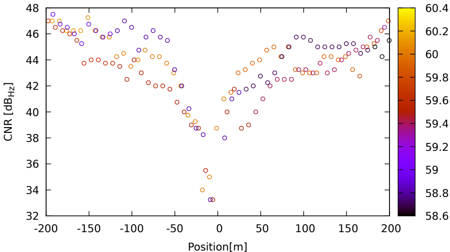
CNR vs position for E19 (E5a) on LeicaGS18 - DOY 263 jam. 1
