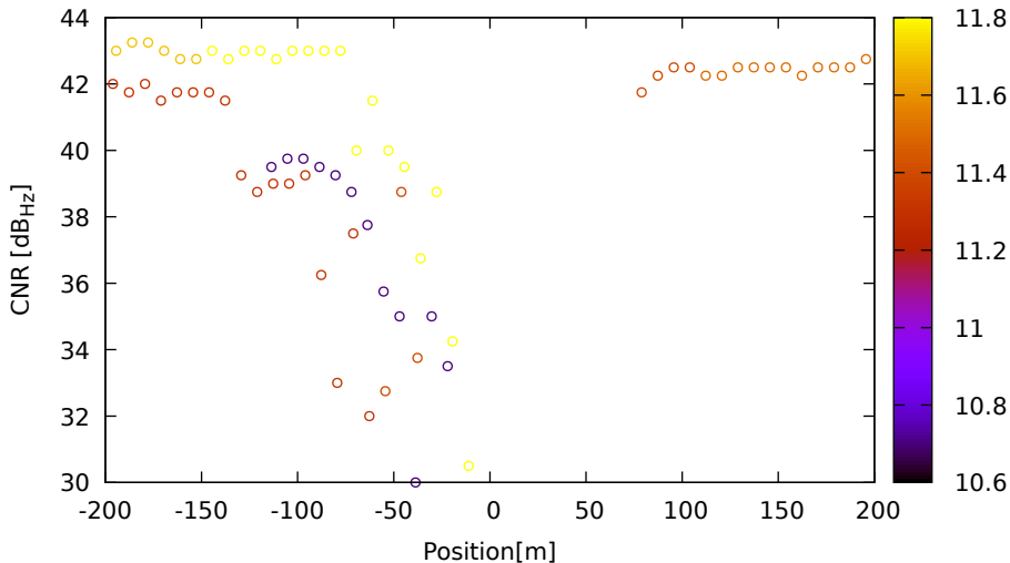
CNR vs position for E36 (E1) on LeicaGS18 - DOY 263 jam. 3
