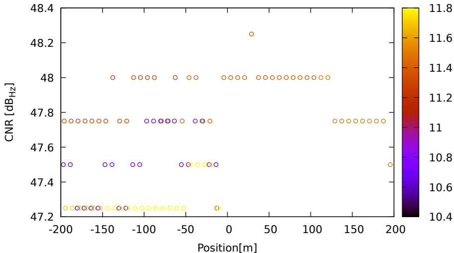
CNR vs position for E36 (E5) on LeicaGS18 - DOY 263 jam. 3
