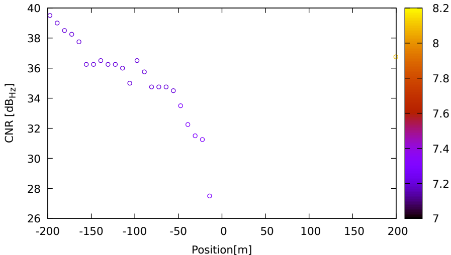
CNR vs position for E36 (E5a) on LeicaGS18 - DOY 263 jam. 1
