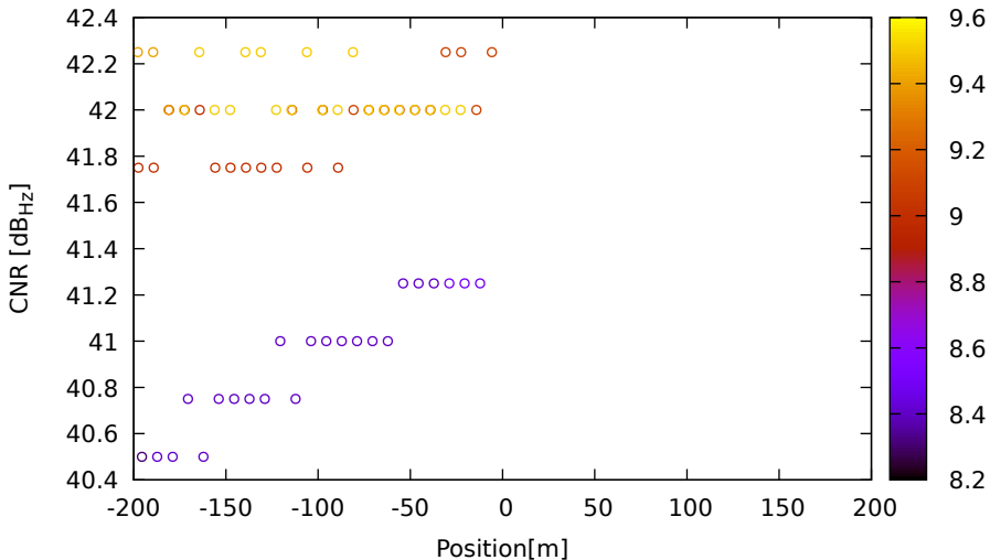
CNR vs position for E36 (E5a) on LeicaGS18 - DOY 263 jam. 2
