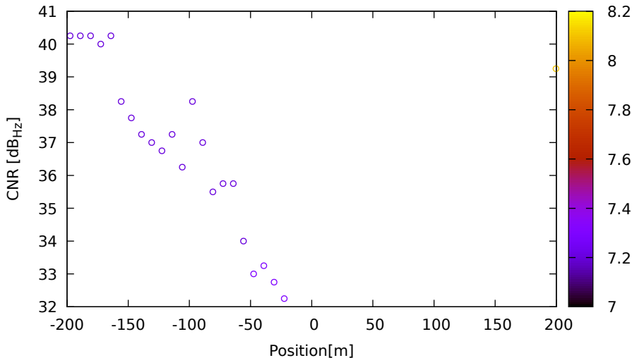
CNR vs position for E36 (E5b) on LeicaGS18 - DOY 263 jam. 1
