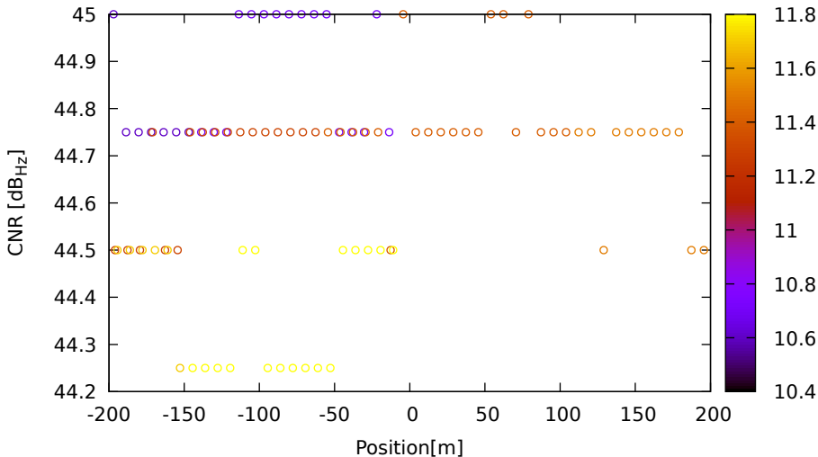
CNR vs position for E36 (E5b) on LeicaGS18 - DOY 263 jam. 3
