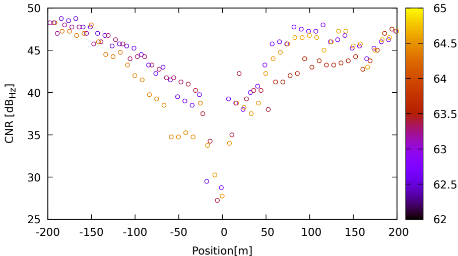
CNR vs position for G04 (L2) on LeicaGS18 - DOY 263 jam. 1
