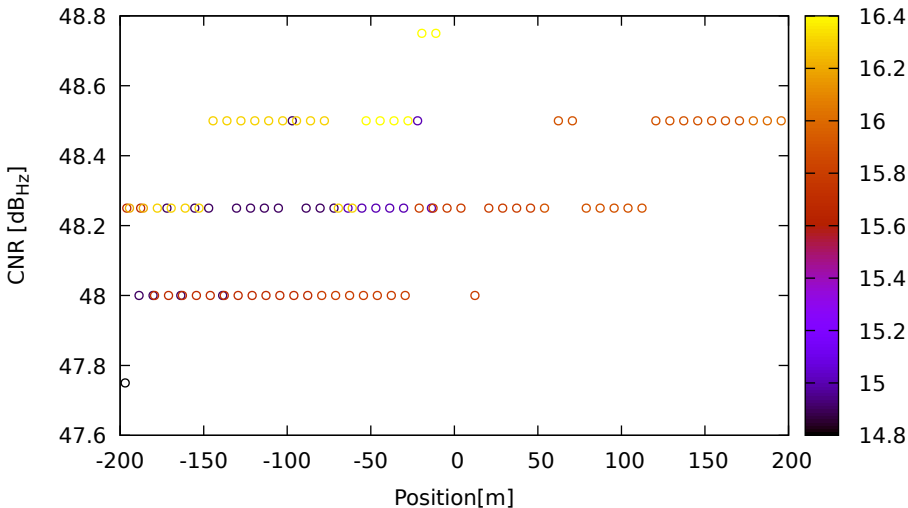
CNR vs position for G06 (L5) on LeicaGS18 - DOY 263 jam. 3
