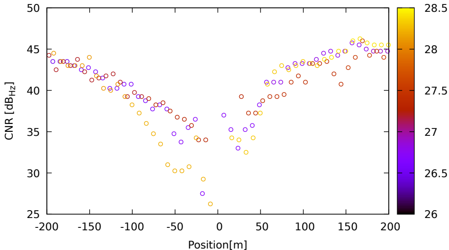
CNR vs position for G09 (L1) on LeicaGS18 - DOY 263 jam. 1
