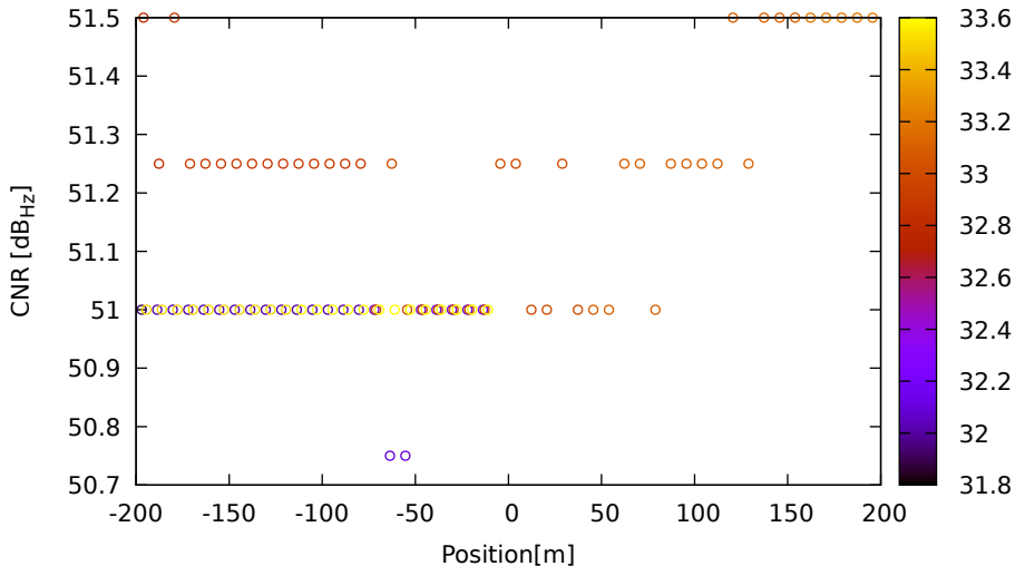
CNR vs position for G09 (L5) on LeicaGS18 - DOY 263 jam. 3
