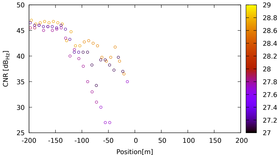
CNR vs position for G21 (L1) on LeicaGS18 - DOY 263 jam. 2
