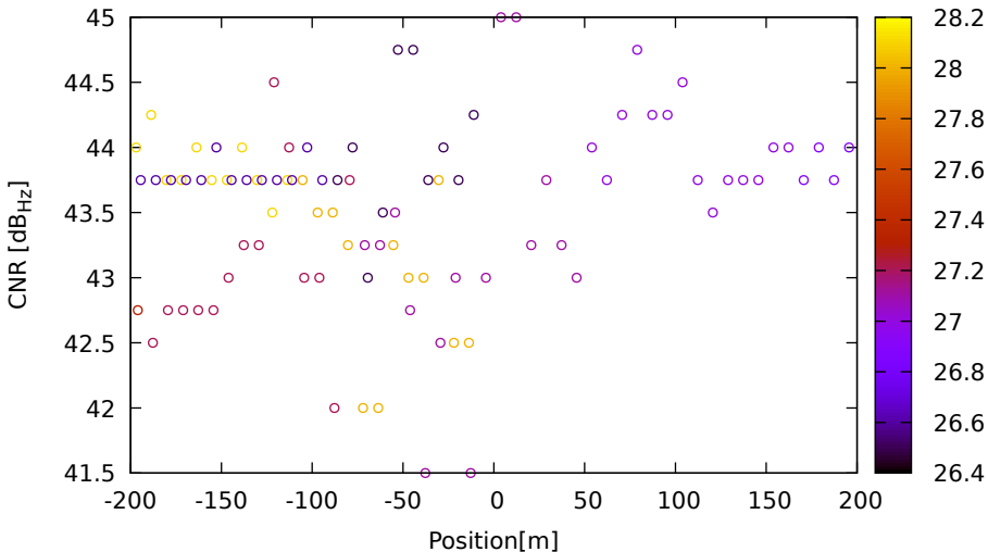
CNR vs position for R01 (G1) on LeicaGS18 - DOY 263 jam. 3
