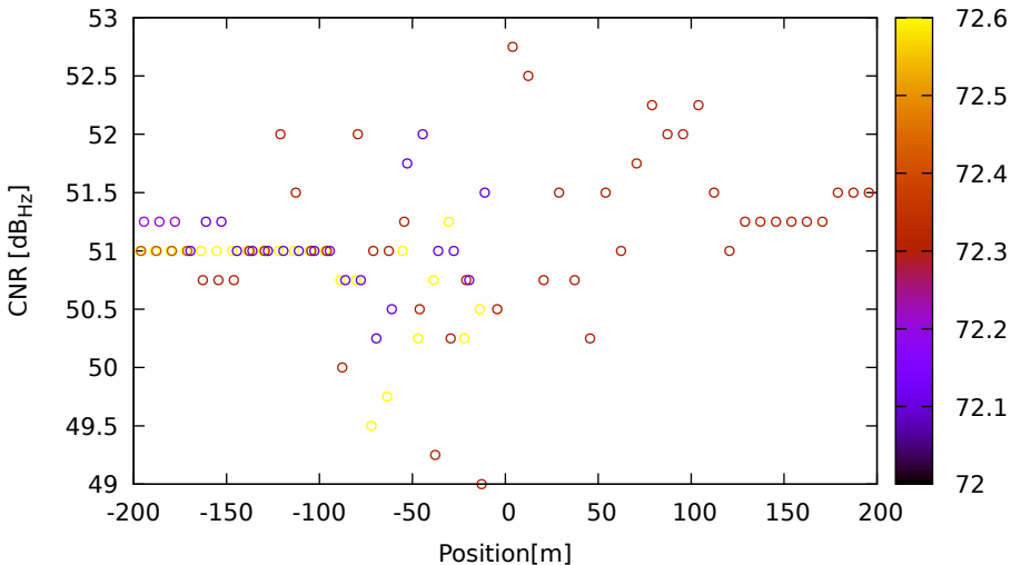
CNR vs position for R02 (G1) on LeicaGS18 - DOY 263 jam. 3
