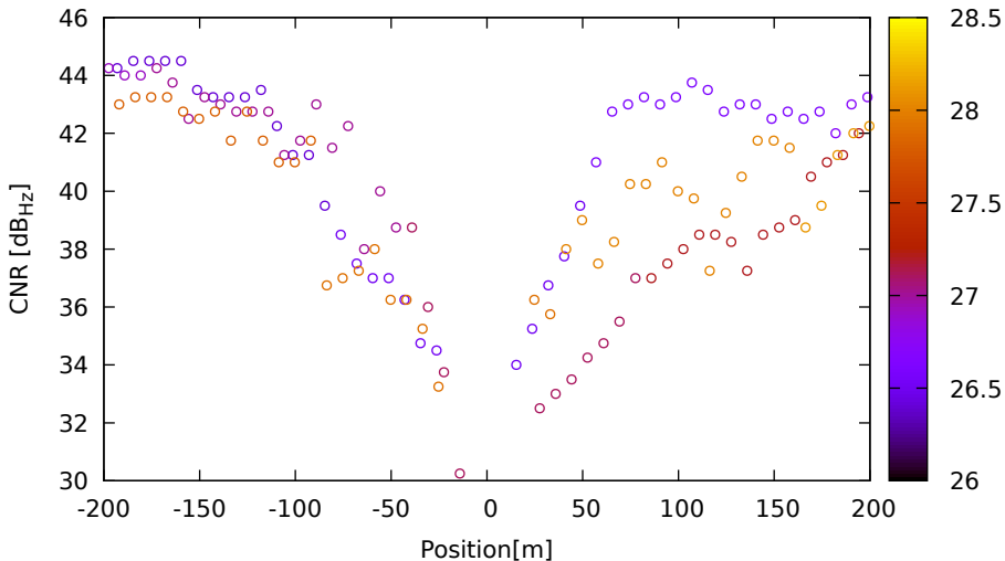
CNR vs position for R03 (G2) on LeicaGS18 - DOY 263 jam. 1
