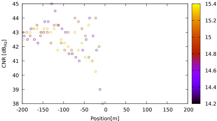
CNR vs position for R11 (G1) on LeicaGS18 - DOY 263 jam. 2
