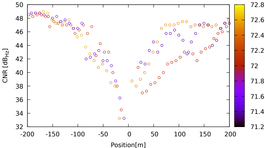
CNR vs position for R17 (G2) on LeicaGS18 - DOY 263 jam. 1
