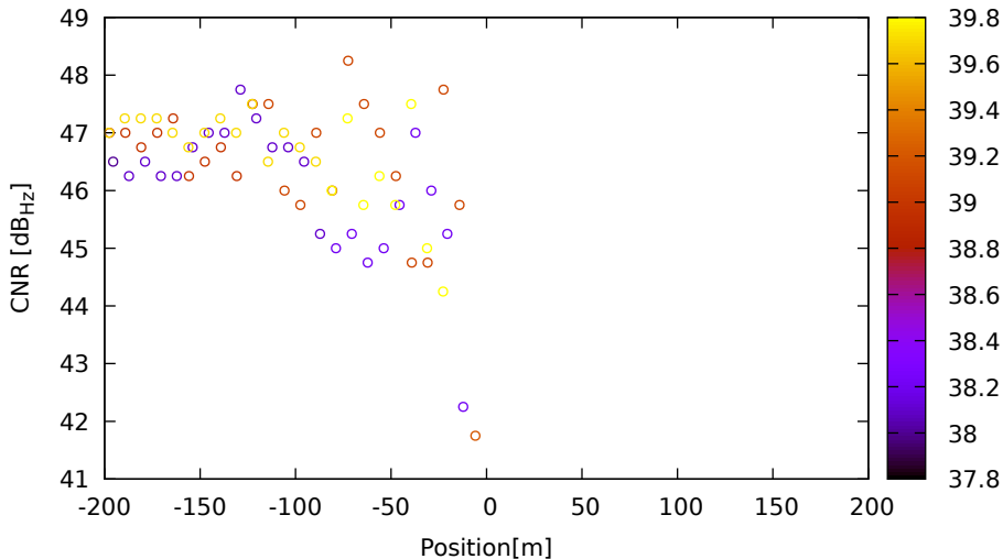
CNR vs position for R18 (G1) on LeicaGS18 - DOY 263 jam. 2
